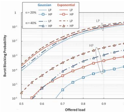
Fig 4. Burst blocking probability as a function of \rho comparing Gaussian and Exponential traffic models and different \alpha ( T = 10 \mu\text{s} and W = 32 ).
