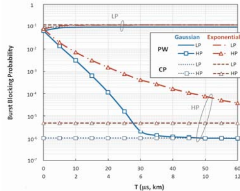
Fig 2. Burst blocking probability as a function of T comparing Gaussian and Exponential traffic models ( \alpha = 30\% , \rho = 0.8 , W = 16 ).
